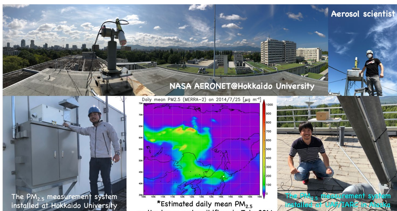
*Fig. 1b of Yasunari et al. (2018, Sci. Rep. , https://doi.org/10.1038/s41598-018-24335-w )
